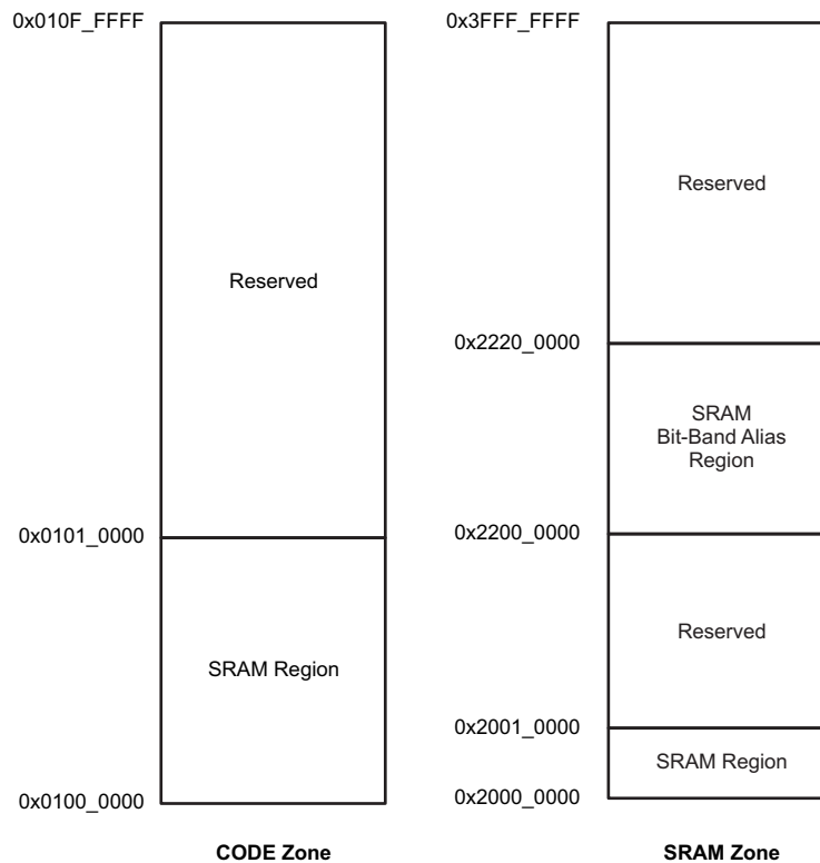
Figure 6-6. SRAM Map
